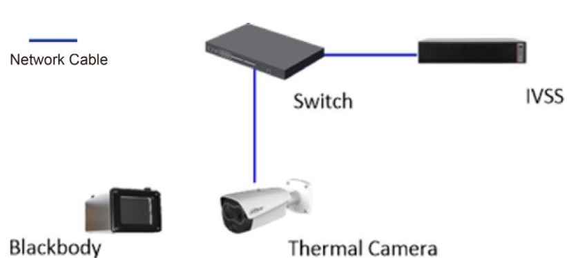
Figure 2-4 TPC-IVSS
