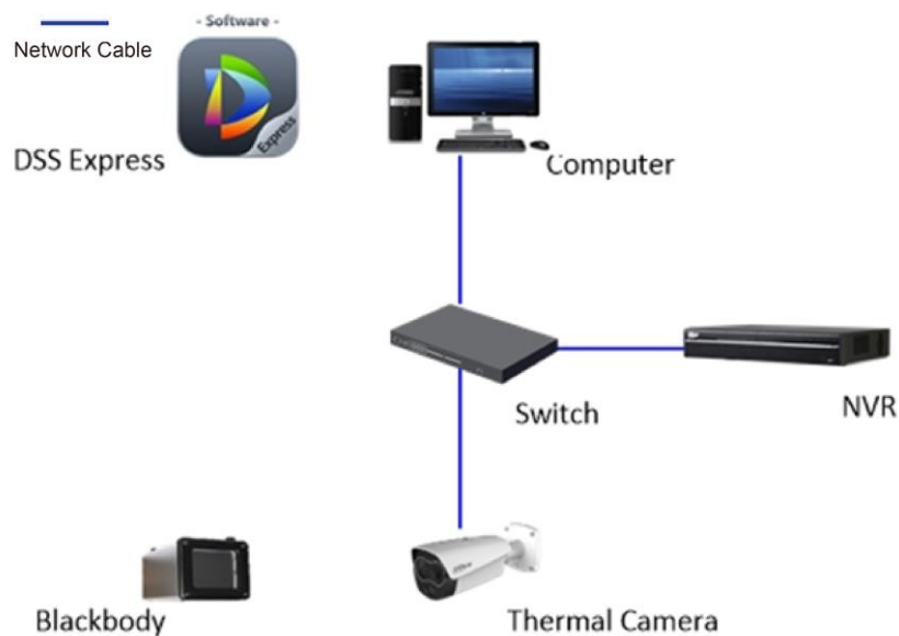
Figure 2-3 TPC-NVR-Express
